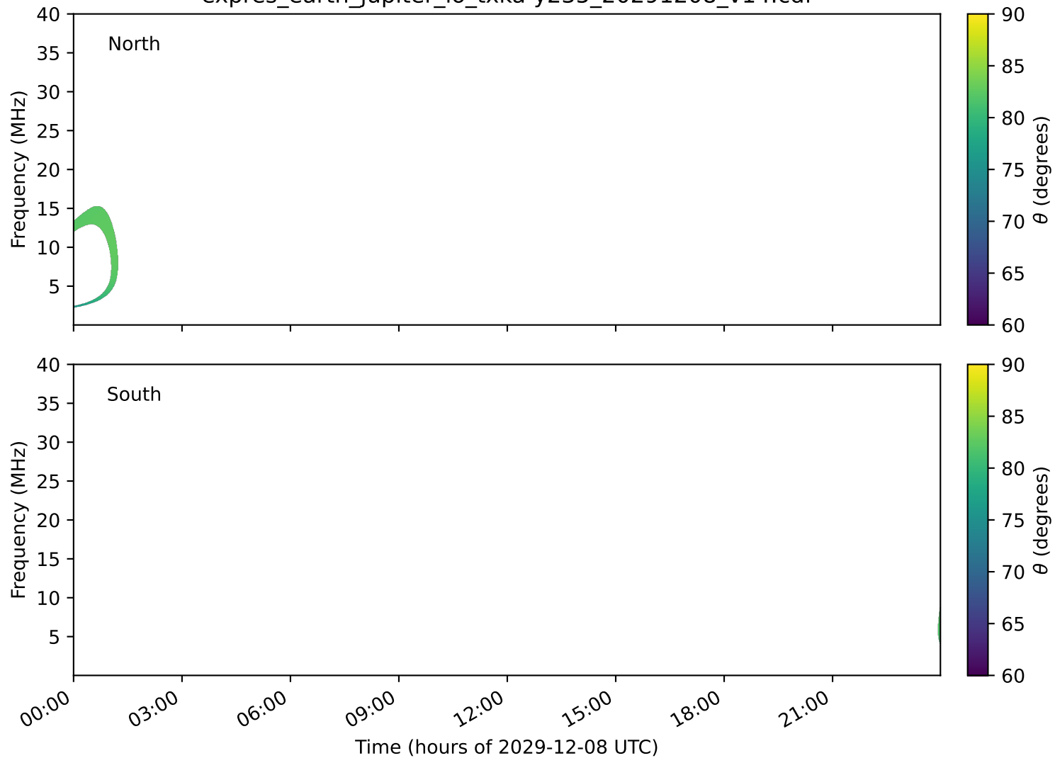
expres_earth_jupiter_io_txka-y235_20291208_v14.cdf
