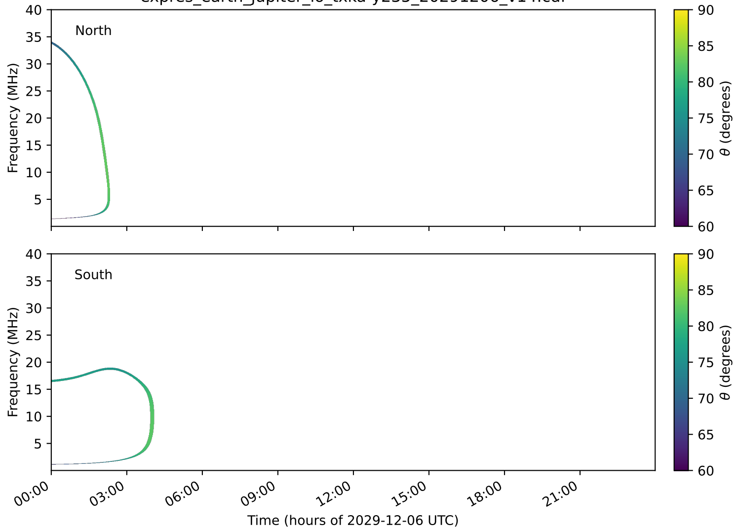
expres_earth_jupiter_io_txka-y235_20291206_v14.cdf
