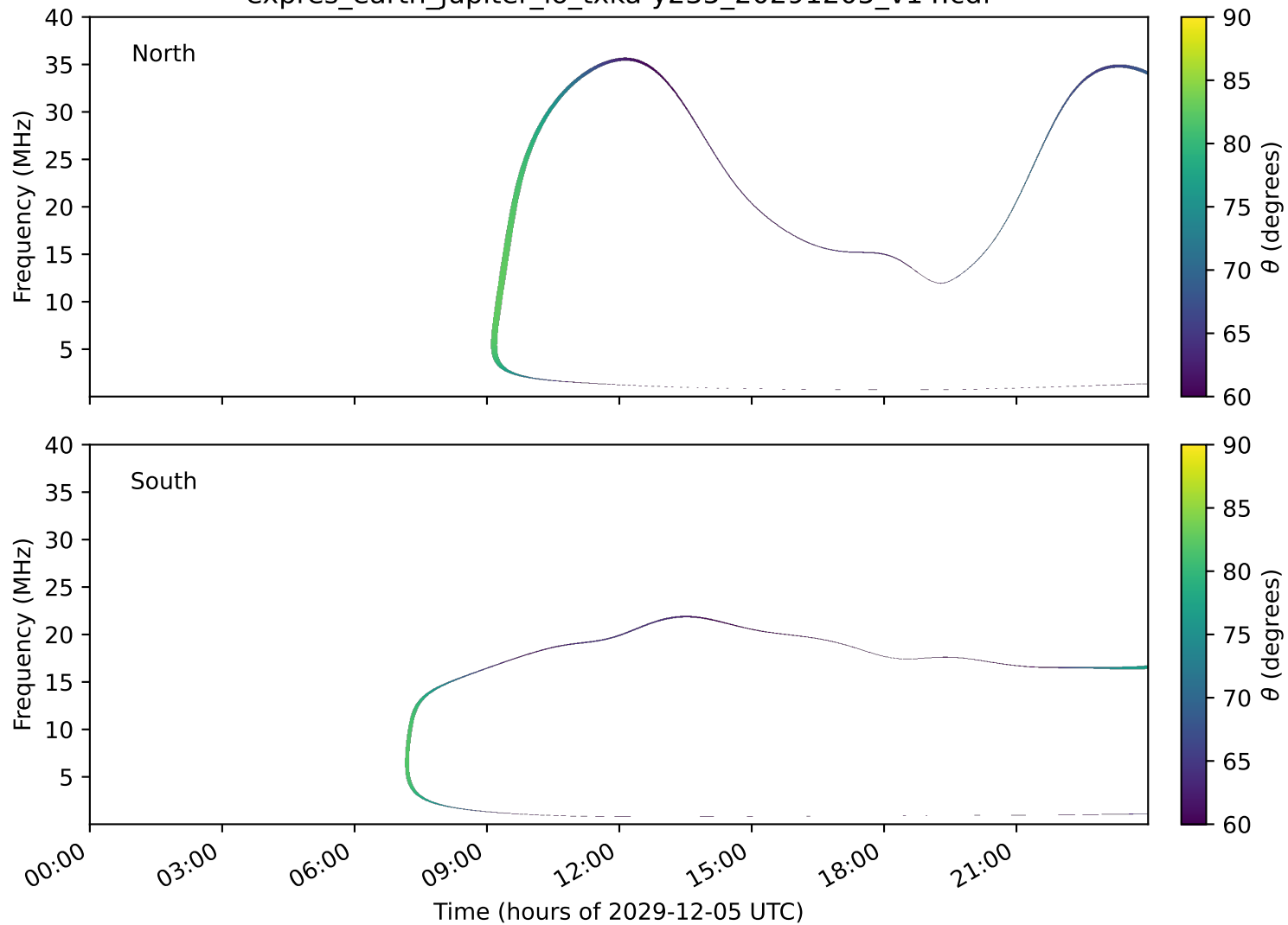
expres_earth_jupiter_io_txka-y235_20291205_v14.cdf
