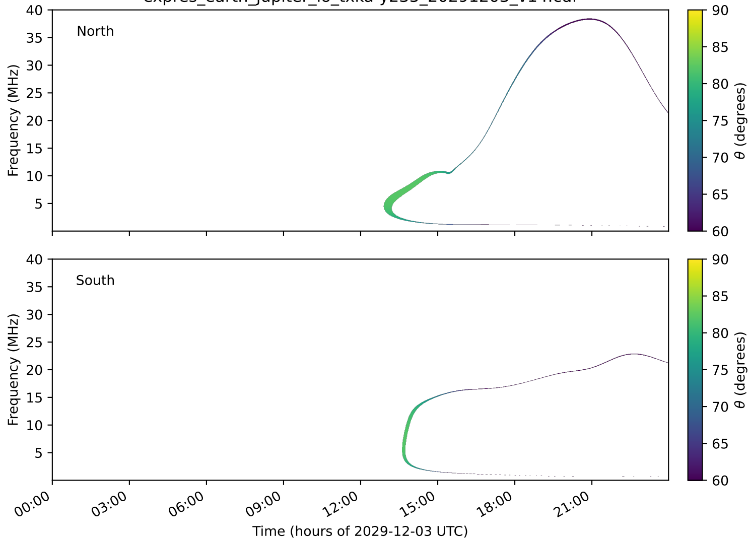
expres_earth_jupiter_io_txka-y235_20291203_v14.cdf
