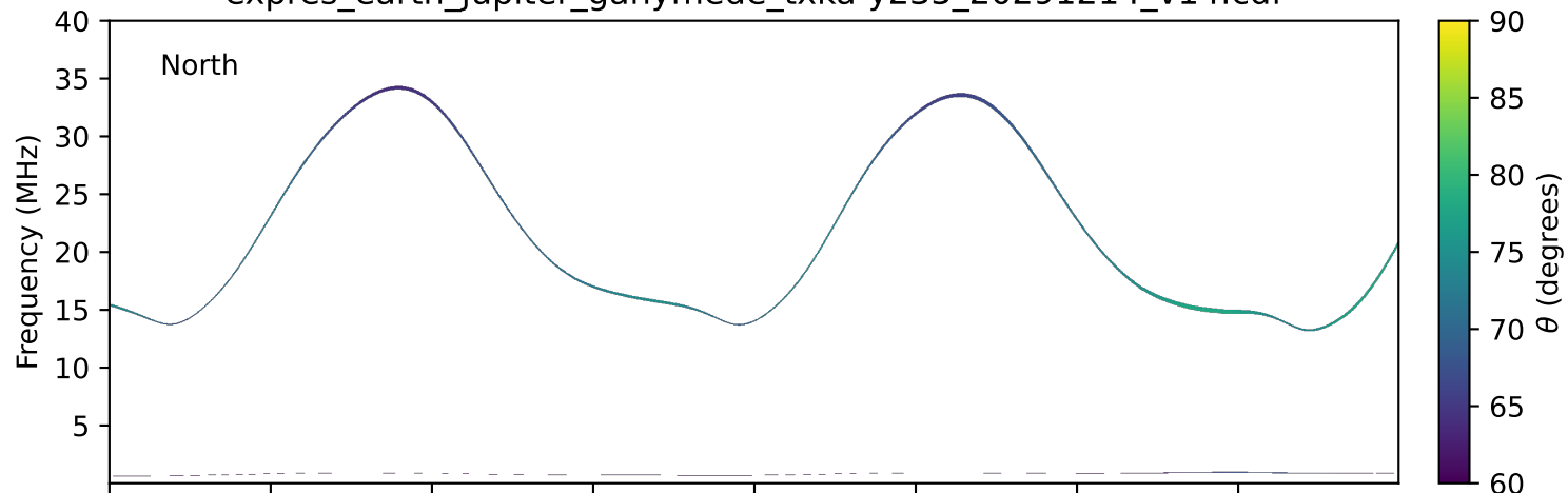
expres_earth_jupiter_ganymede_txka-y235_20291214_v14.cdf
