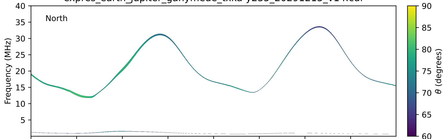
expres_earth_jupiter_ganymede_txka-y235_20291213_v14.cdf
