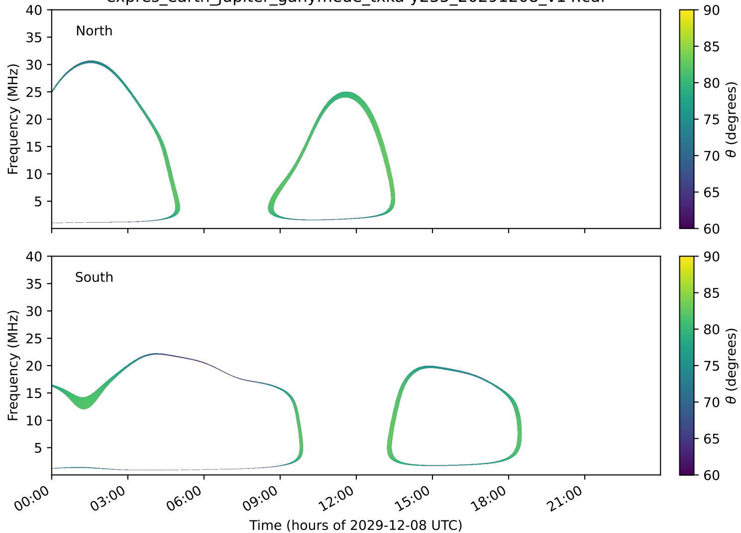
expres_earth_jupiter_ganymede_txka-y235_20291208_v14.cdf
