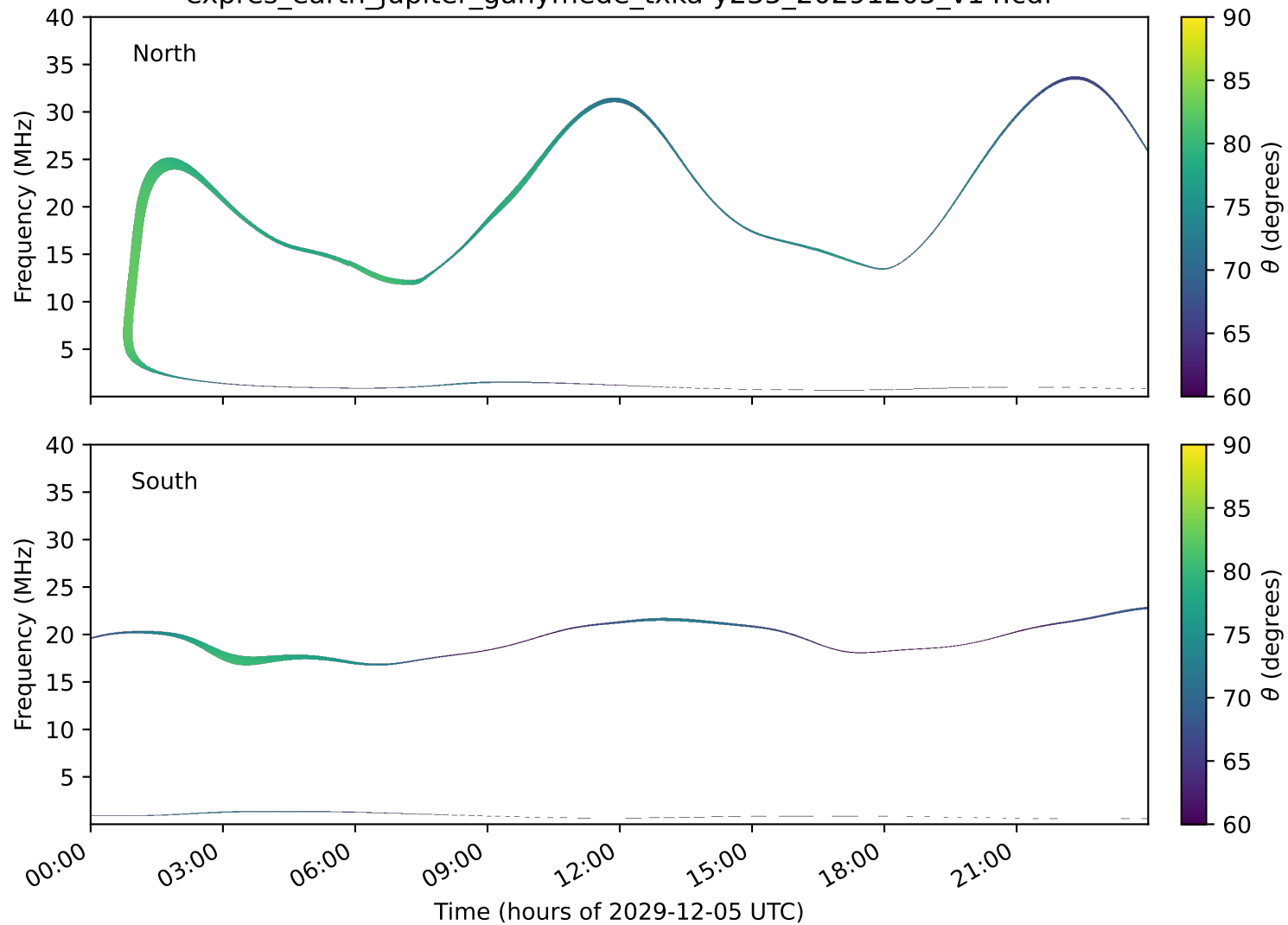
expres_earth_jupiter_ganymede_txka-y235_20291205_v14.cdf
