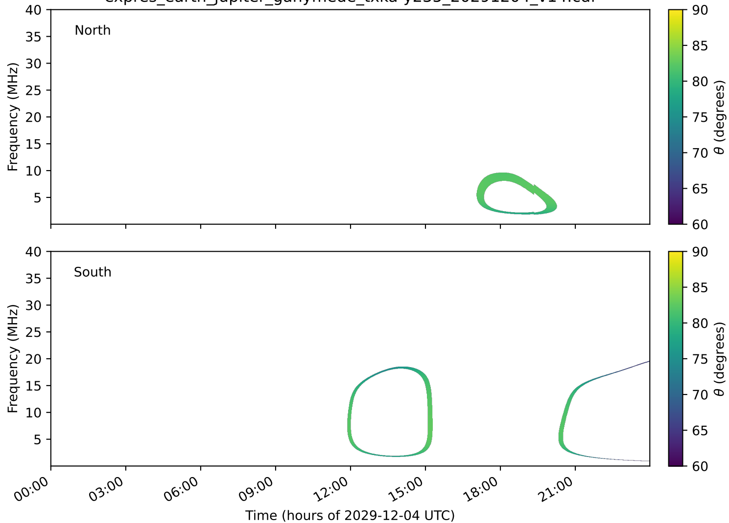
expres_earth_jupiter_ganymede_txka-y235_20291204_v14.cdf
