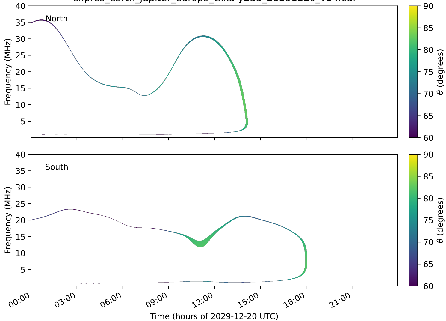
expres_earth_jupiter_europa_txka-y235_20291220_v14.cdf
