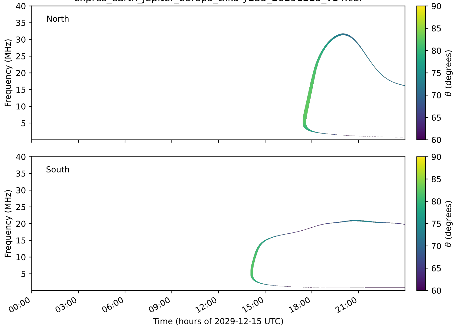
expres_earth_jupiter_europa_txka-y235_20291215_v14.cdf
