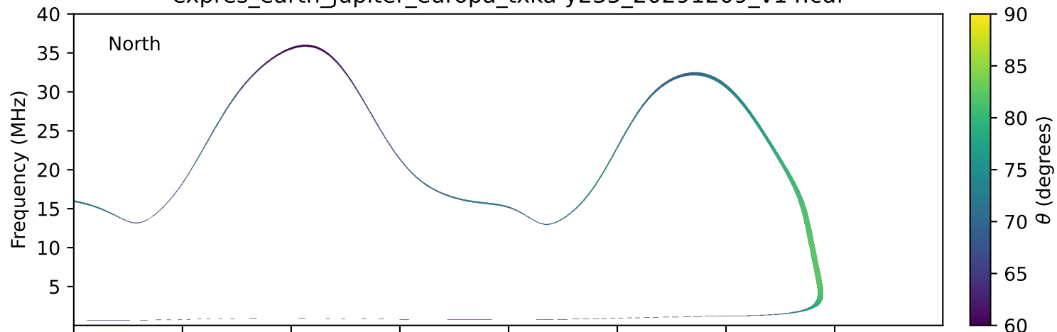
expres_earth_jupiter_europa_txka-y235_20291209_v14.cdf
