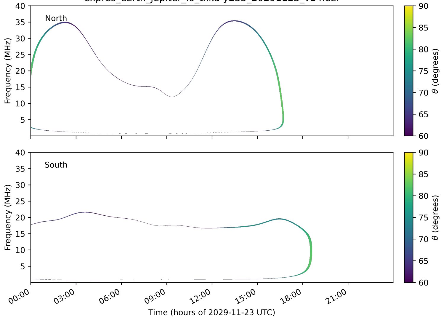
expres_earth_jupiter_io_txka-y235_20291123_v14.cdf
