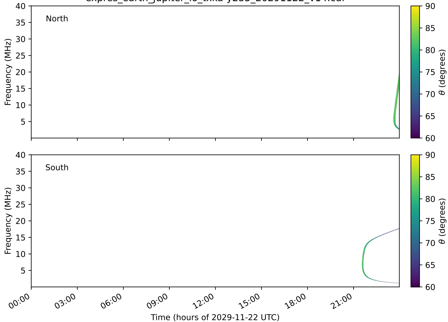
expres_earth_jupiter_io_txka-y235_20291122_v14.cdf
