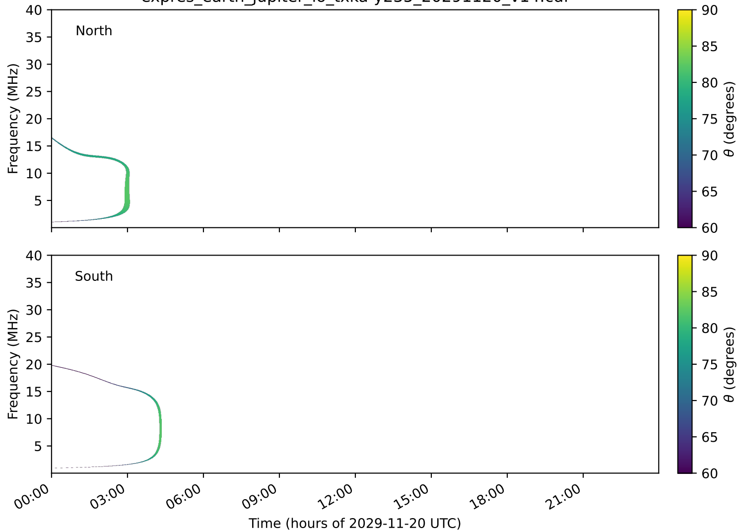
expres_earth_jupiter_io_txka-y235_20291120_v14.cdf
