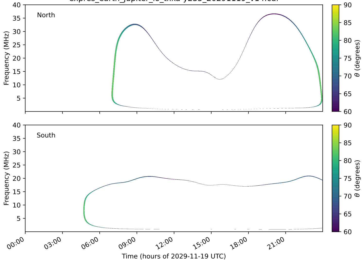
expres_earth_jupiter_io_txka-y235_20291119_v14.cdf
