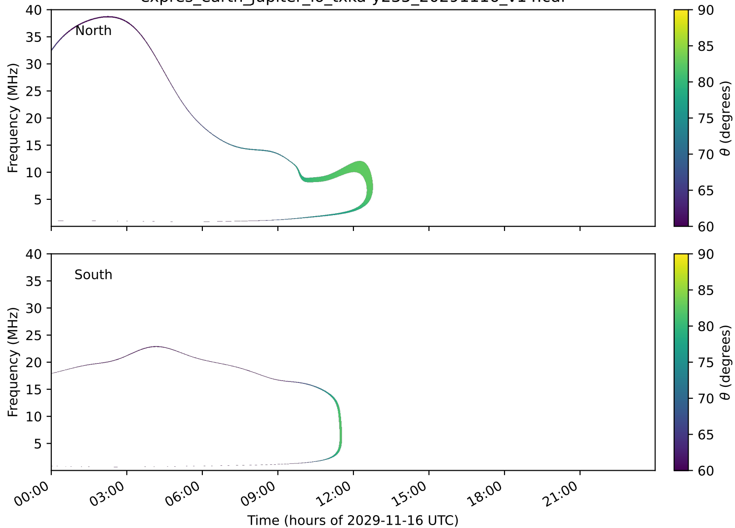
expres_earth_jupiter_io_txka-y235_20291116_v14.cdf
