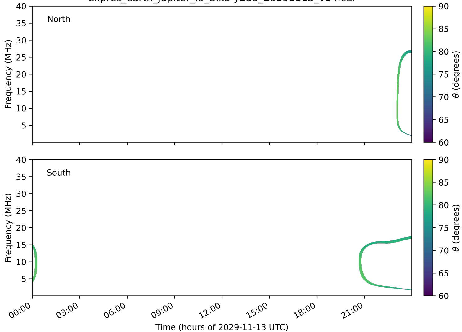
expres_earth_jupiter_io_txka-y235_20291113_v14.cdf
