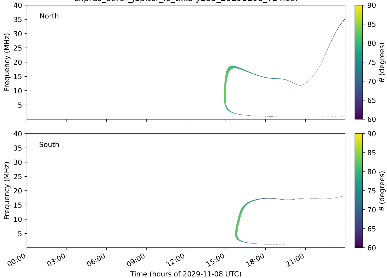
expres_earth_jupiter_io_txka-y235_20291108_v14.cdf
