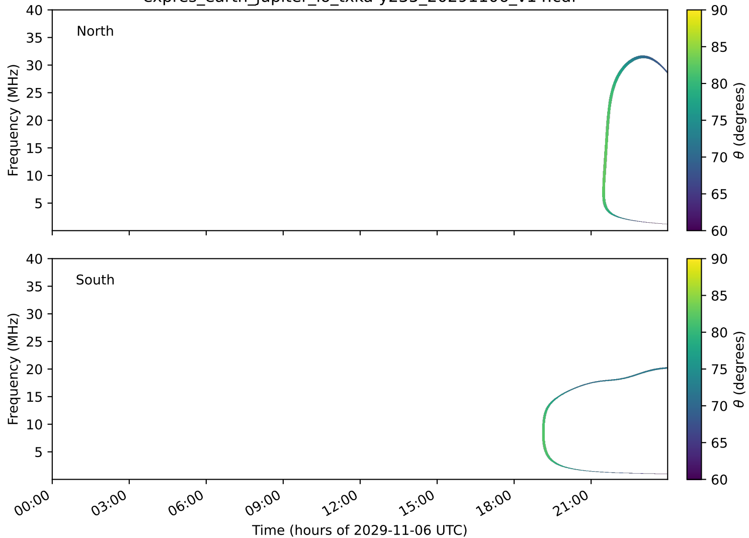
expres_earth_jupiter_io_txka-y235_20291106_v14.cdf
