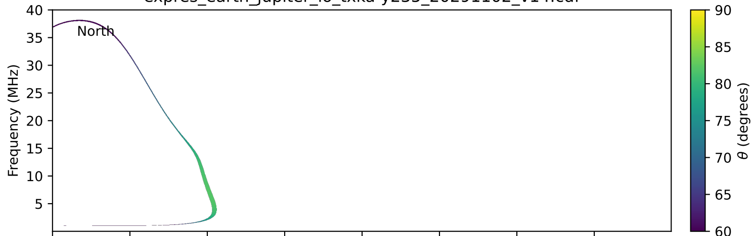
expres_earth_jupiter_io_txka-y235_20291102_v14.cdf
