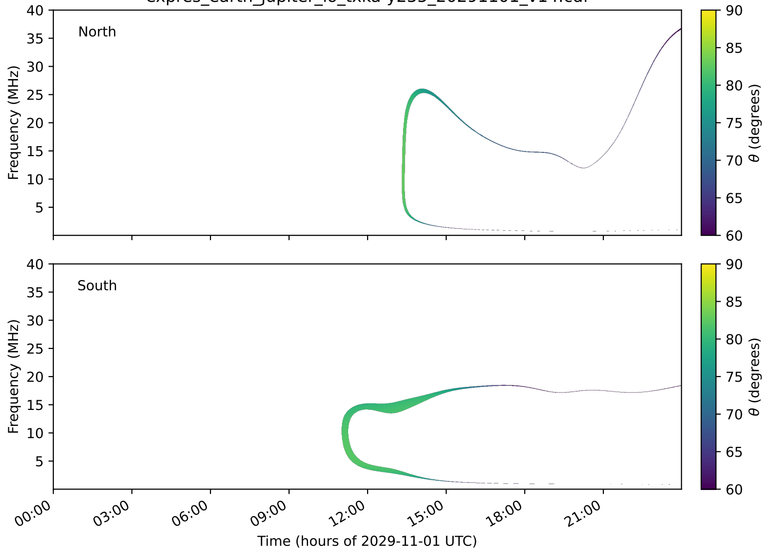
expres_earth_jupiter_io_txka-y235_20291101_v14.cdf
