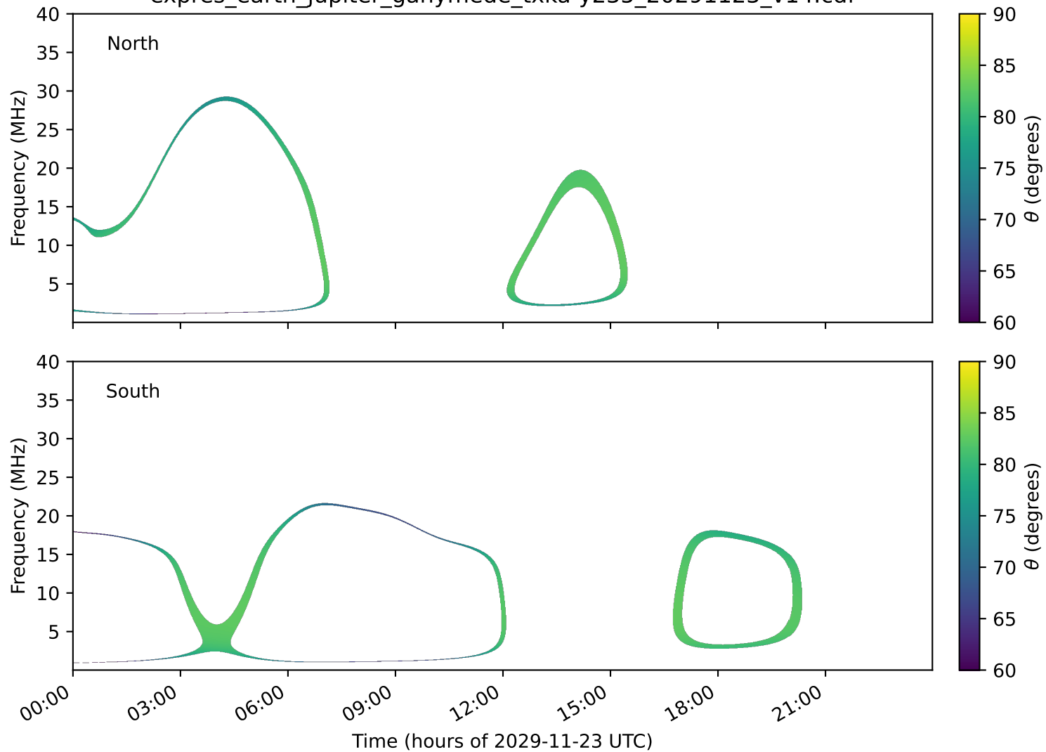
expres_earth_jupiter_ganymede_txka-y235_20291123_v14.cdf
