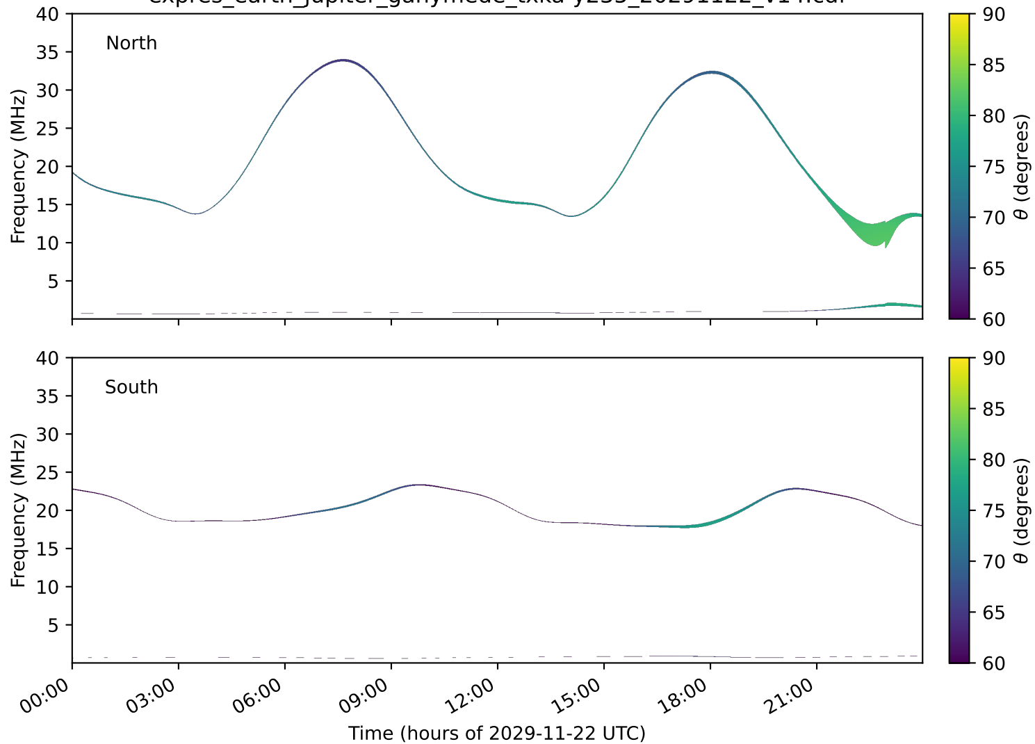
expres_earth_jupiter_ganymede_txka-y235_20291122_v14.cdf
