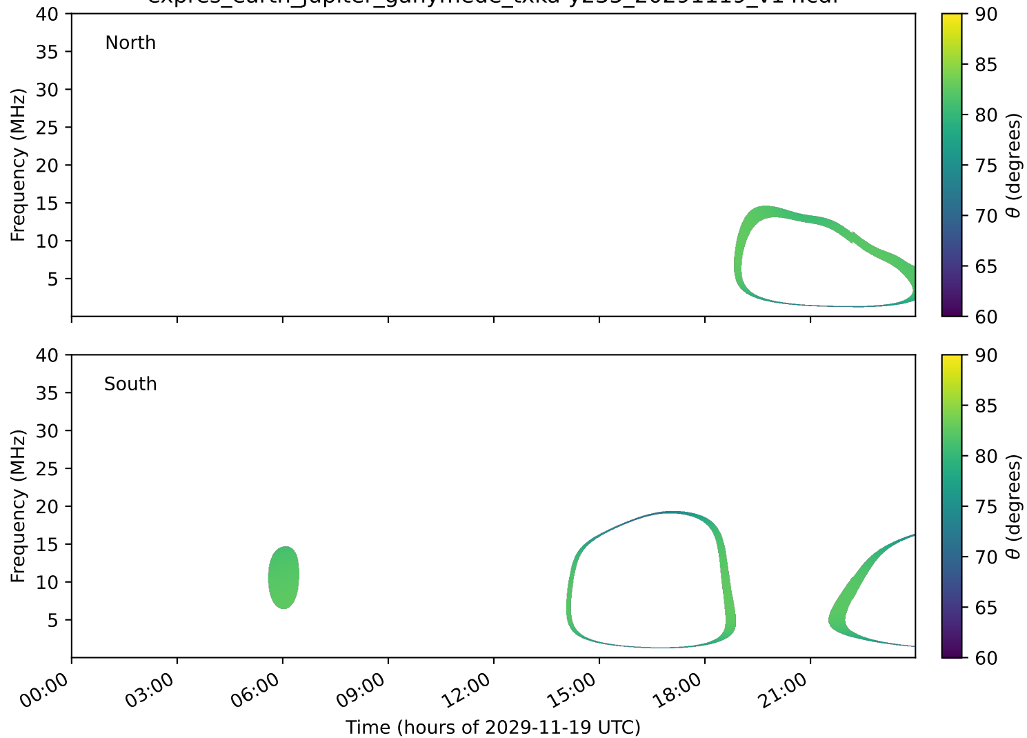
expres_earth_jupiter_ganymede_txka-y235_20291119_v14.cdf
