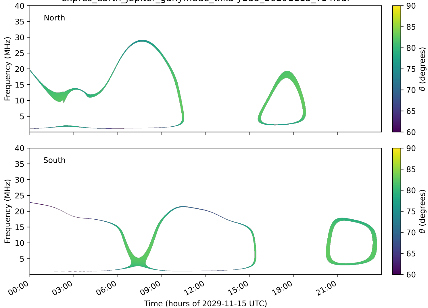
expres_earth_jupiter_ganymede_txka-y235_20291115_v14.cdf
