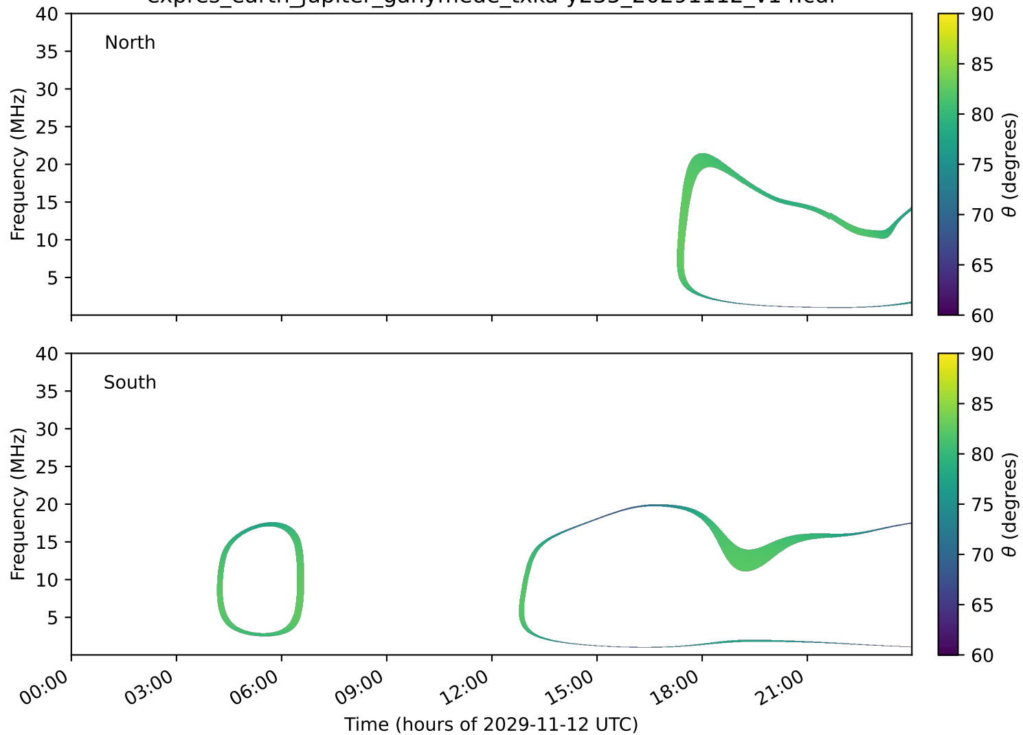
expres_earth_jupiter_ganymede_txka-y235_20291112_v14.cdf
