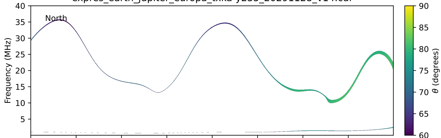
expres_earth_jupiter_europa_txka-y235_20291128_v14.cdf
