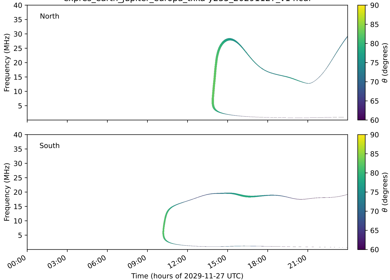
expres_earth_jupiter_europa_txka-y235_20291127_v14.cdf
