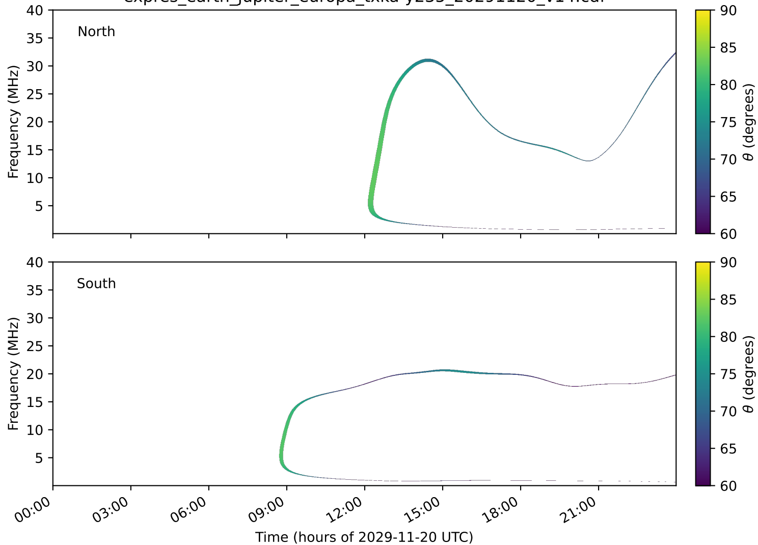
expres_earth_jupiter_europa_txka-y235_20291120_v14.cdf
