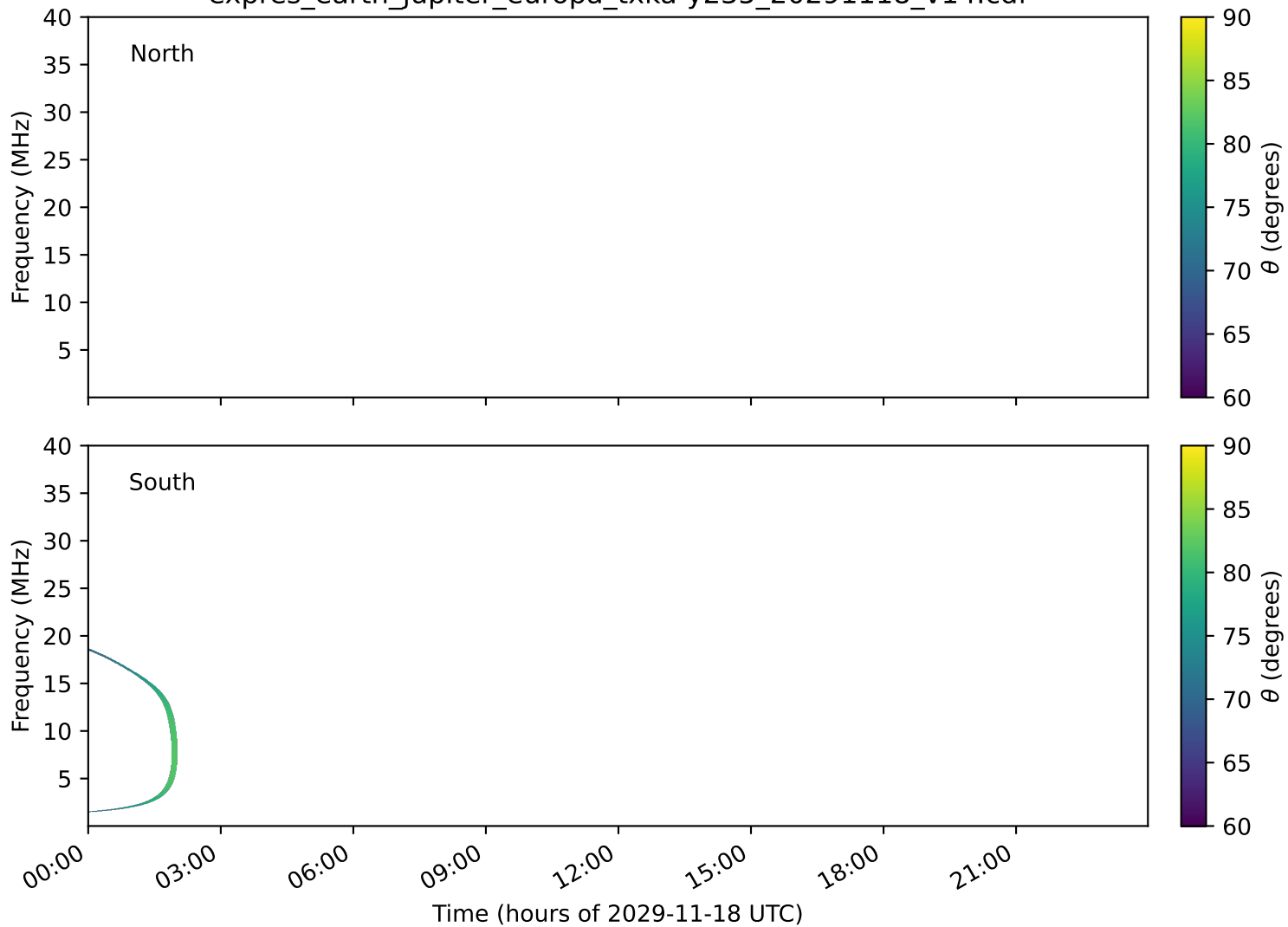
expres_earth_jupiter_europa_txka-y235_20291118_v14.cdf
