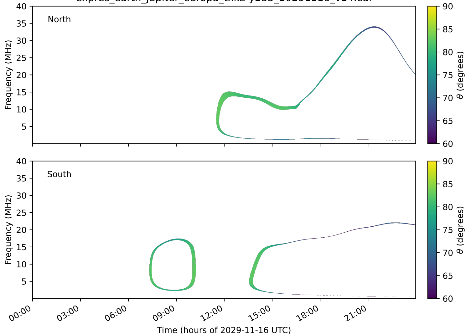
expres_earth_jupiter_europa_txka-y235_20291116_v14.cdf
