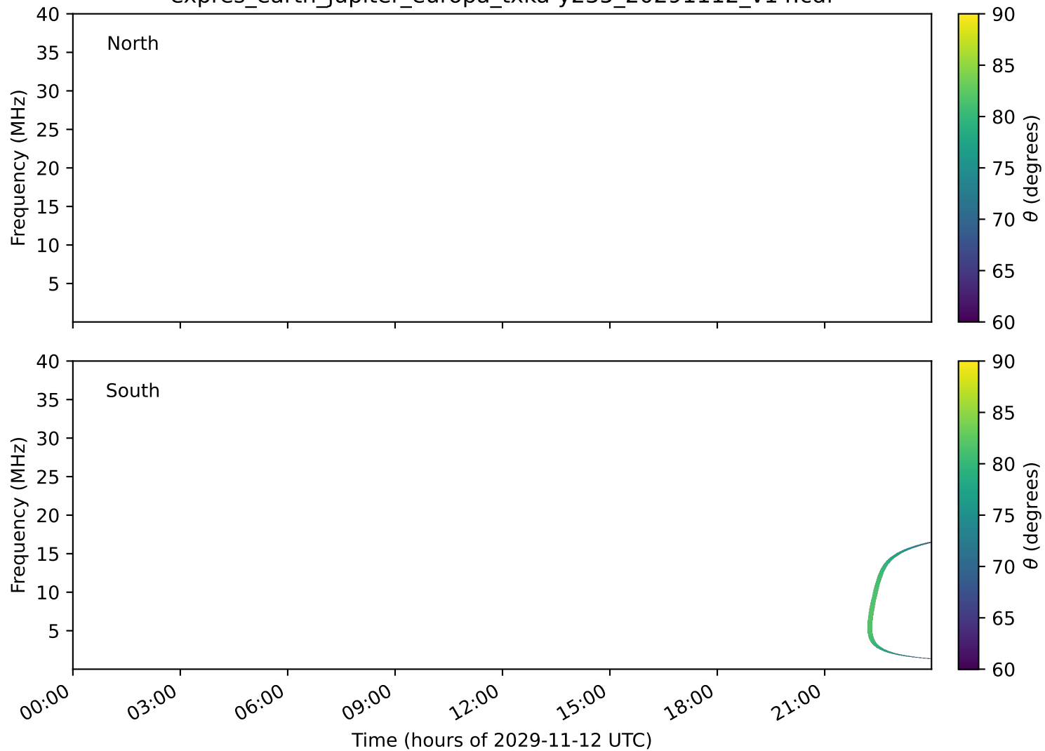
expres_earth_jupiter_europa_txka-y235_20291112_v14.cdf
