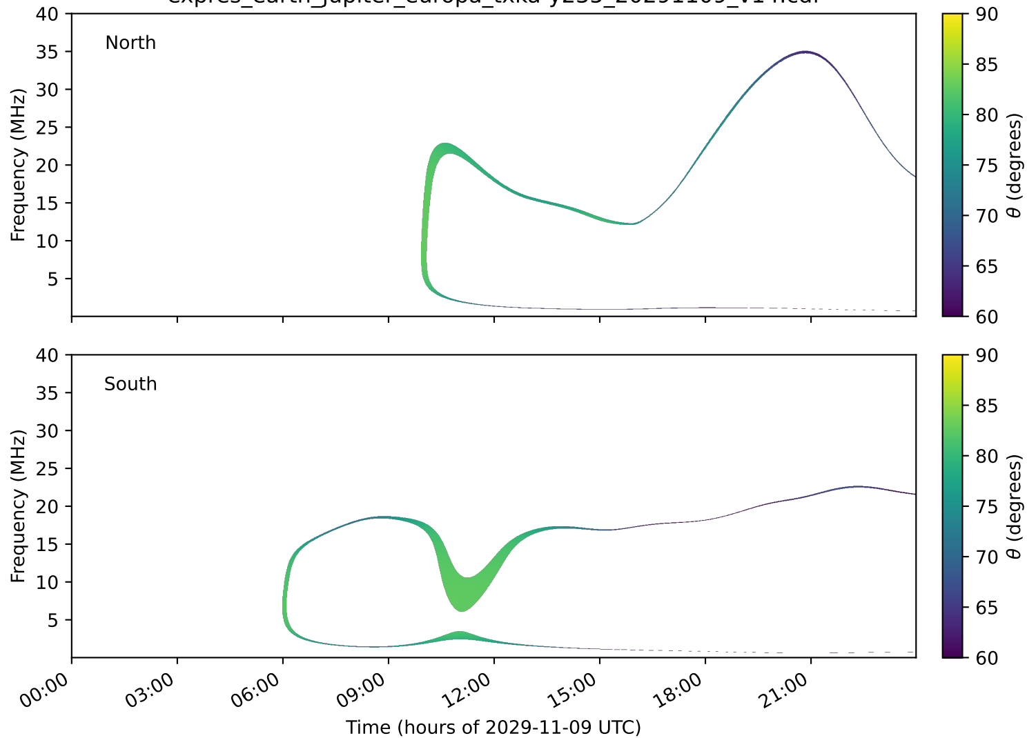
expres_earth_jupiter_europa_txka-y235_20291109_v14.cdf
