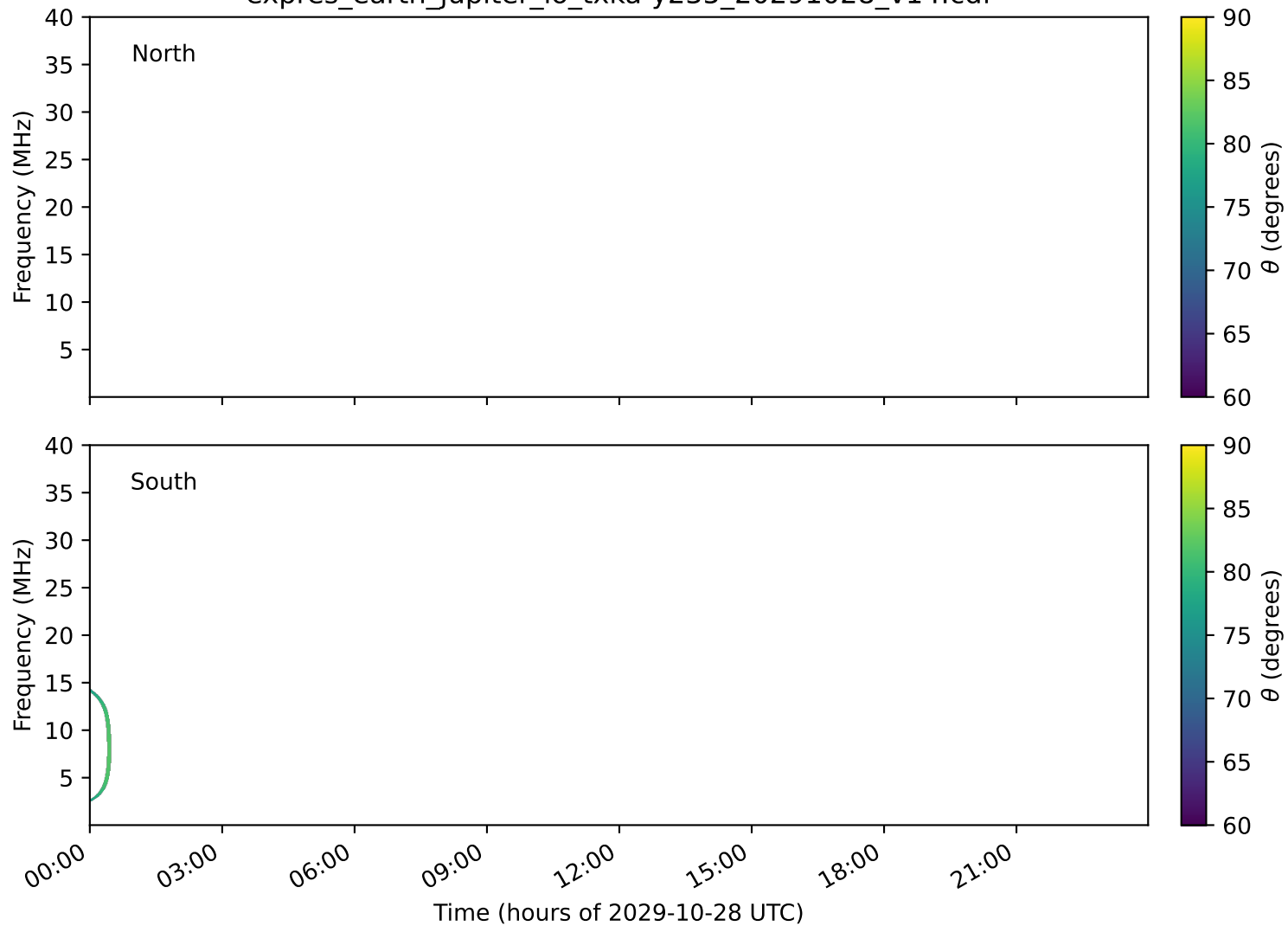
expres_earth_jupiter_io_txka-y235_20291028_v14.cdf
