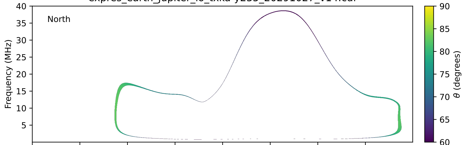
expres_earth_jupiter_io_txka-y235_20291027_v14.cdf
