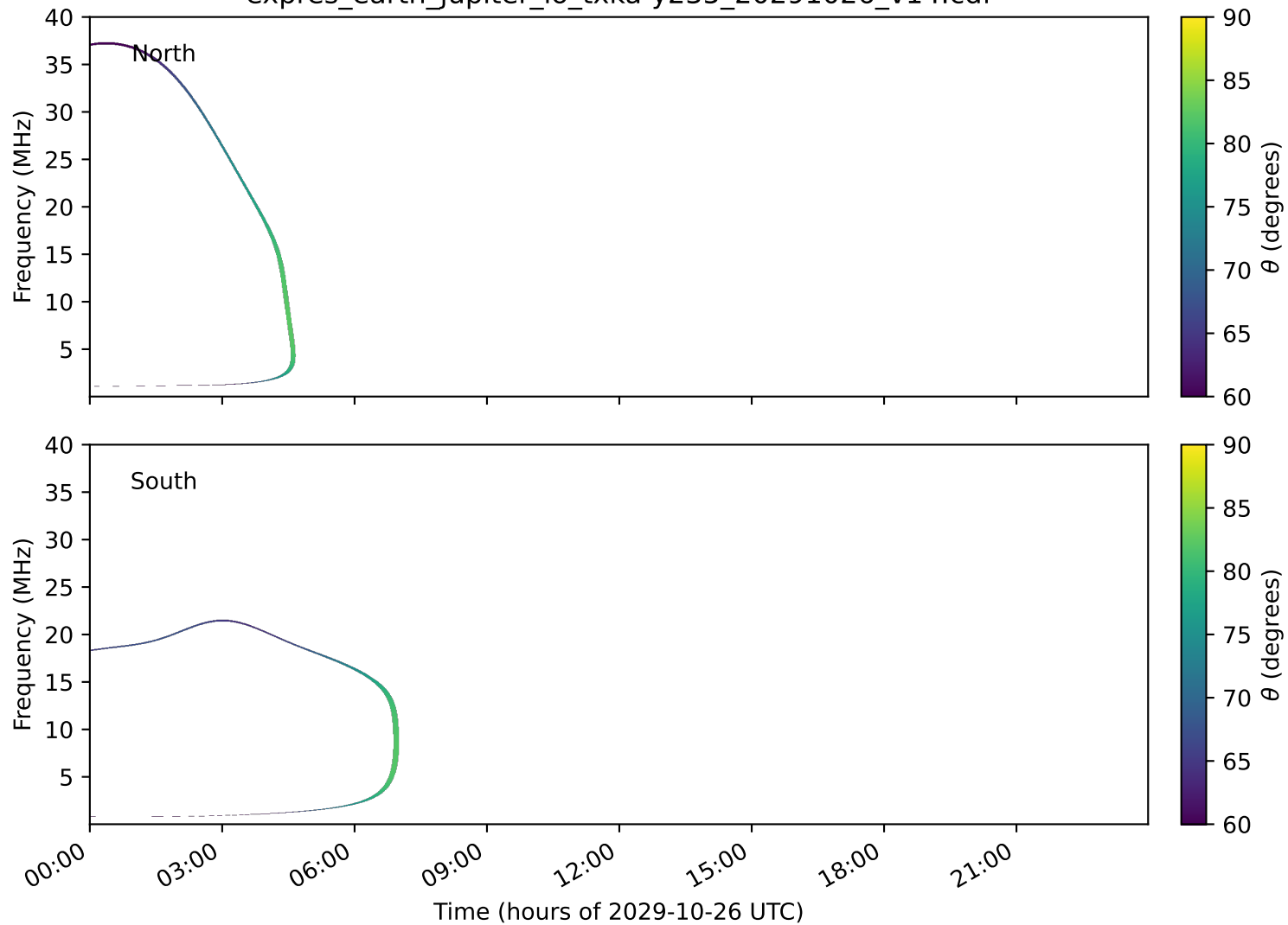
expres_earth_jupiter_io_txka-y235_20291026_v14.cdf
