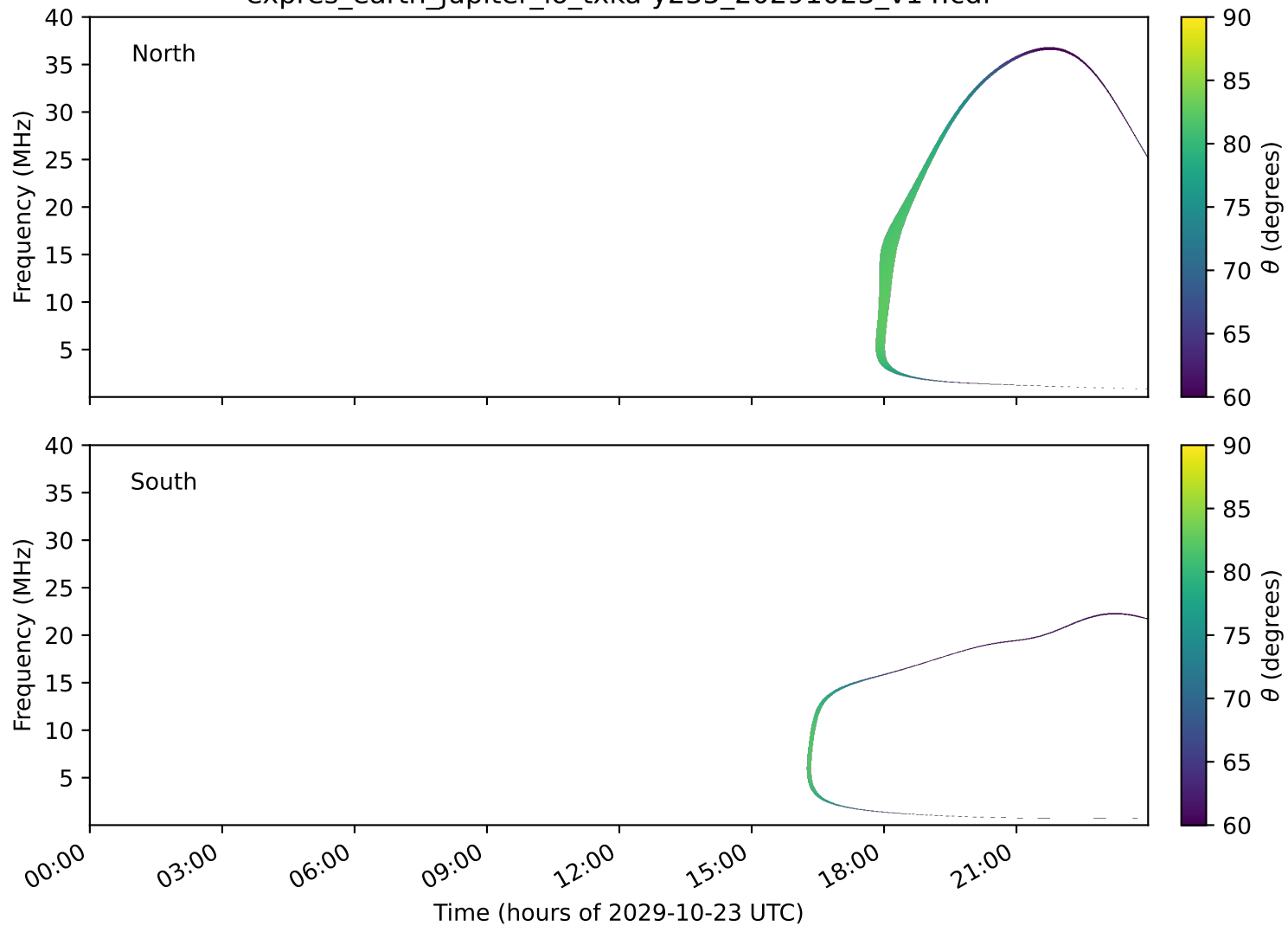
expres_earth_jupiter_io_txka-y235_20291023_v14.cdf
