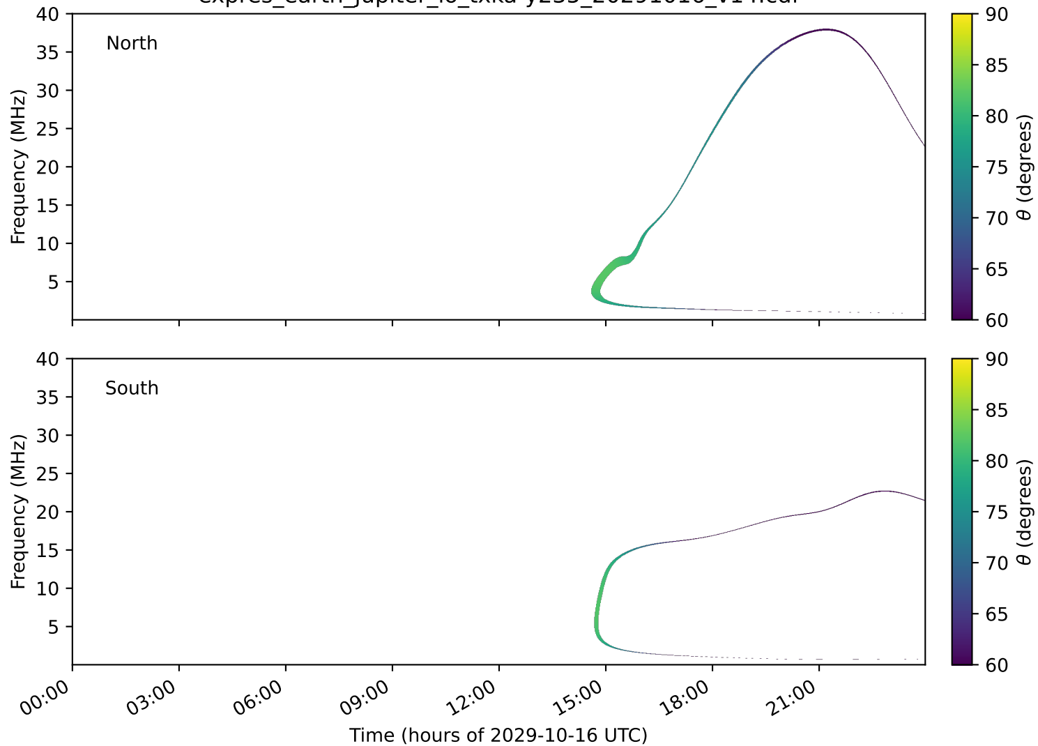
expres_earth_jupiter_io_txka-y235_20291016_v14.cdf
