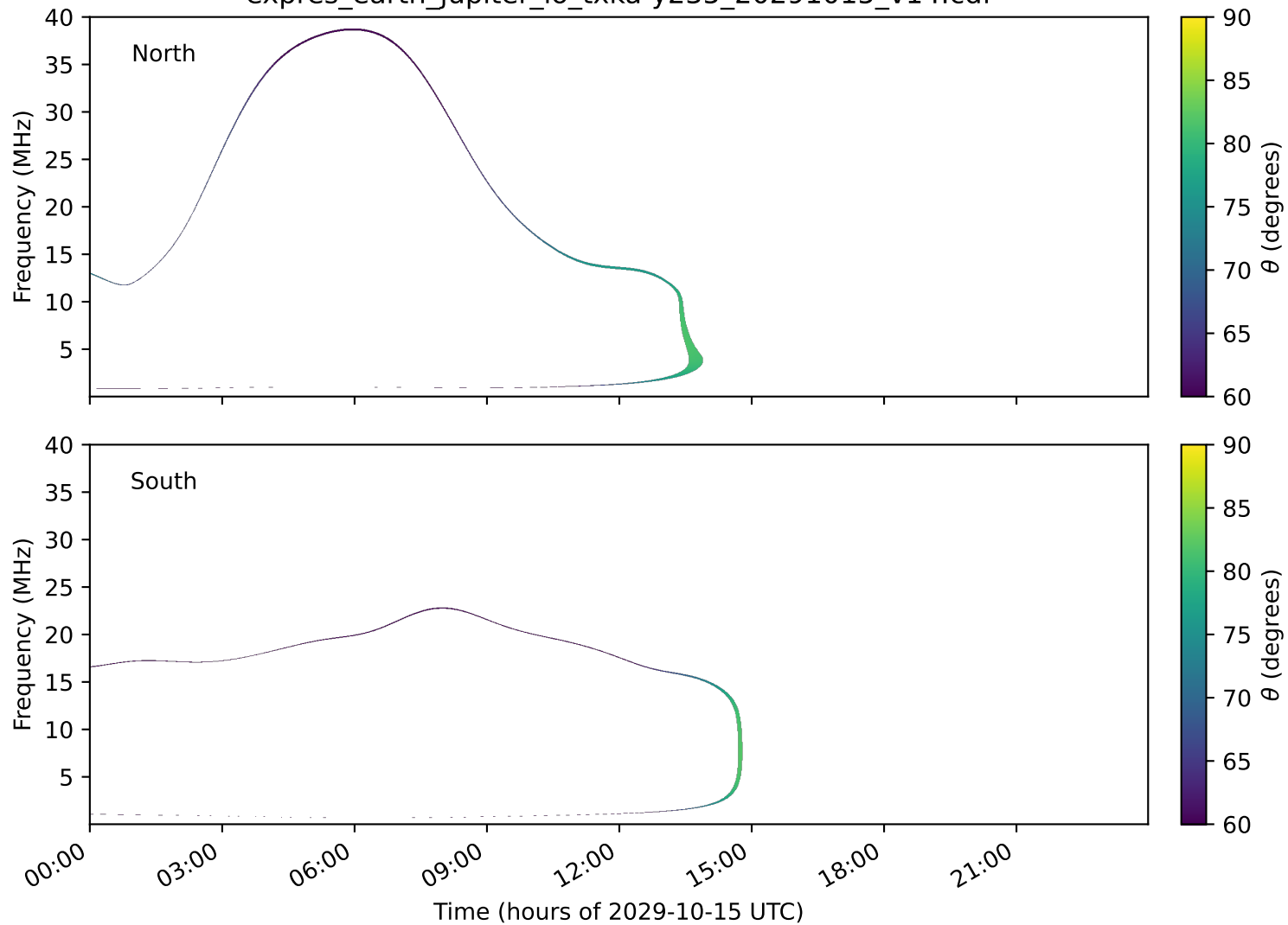
expres_earth_jupiter_io_txka-y235_20291015_v14.cdf
