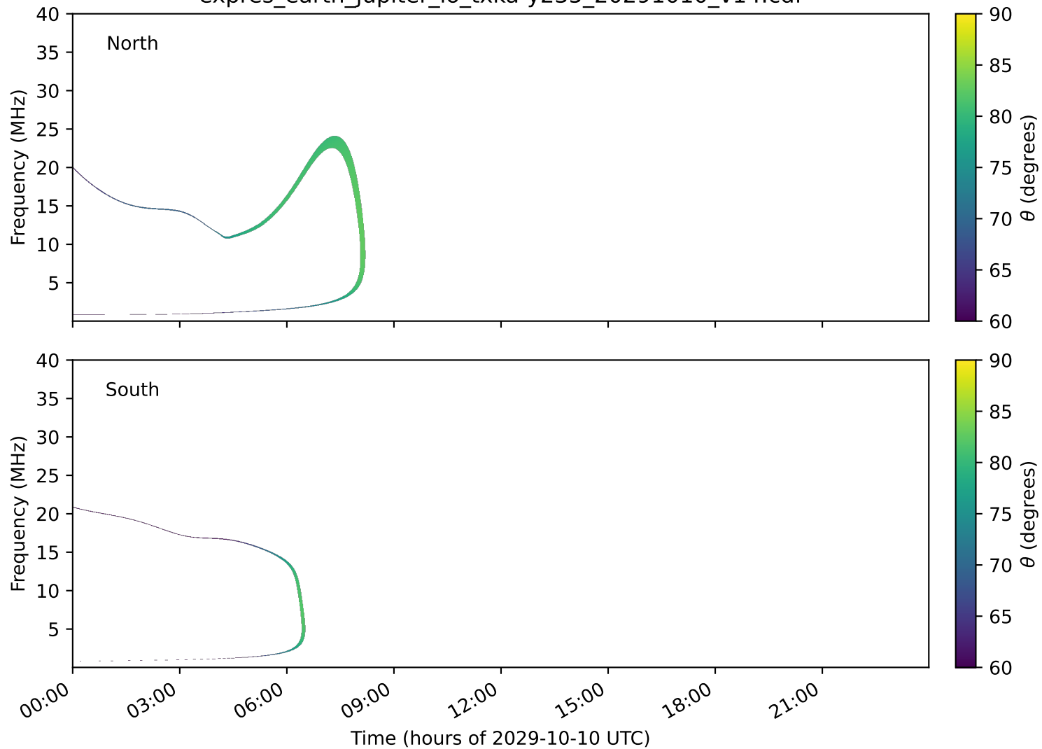
expres_earth_jupiter_io_txka-y235_20291010_v14.cdf
