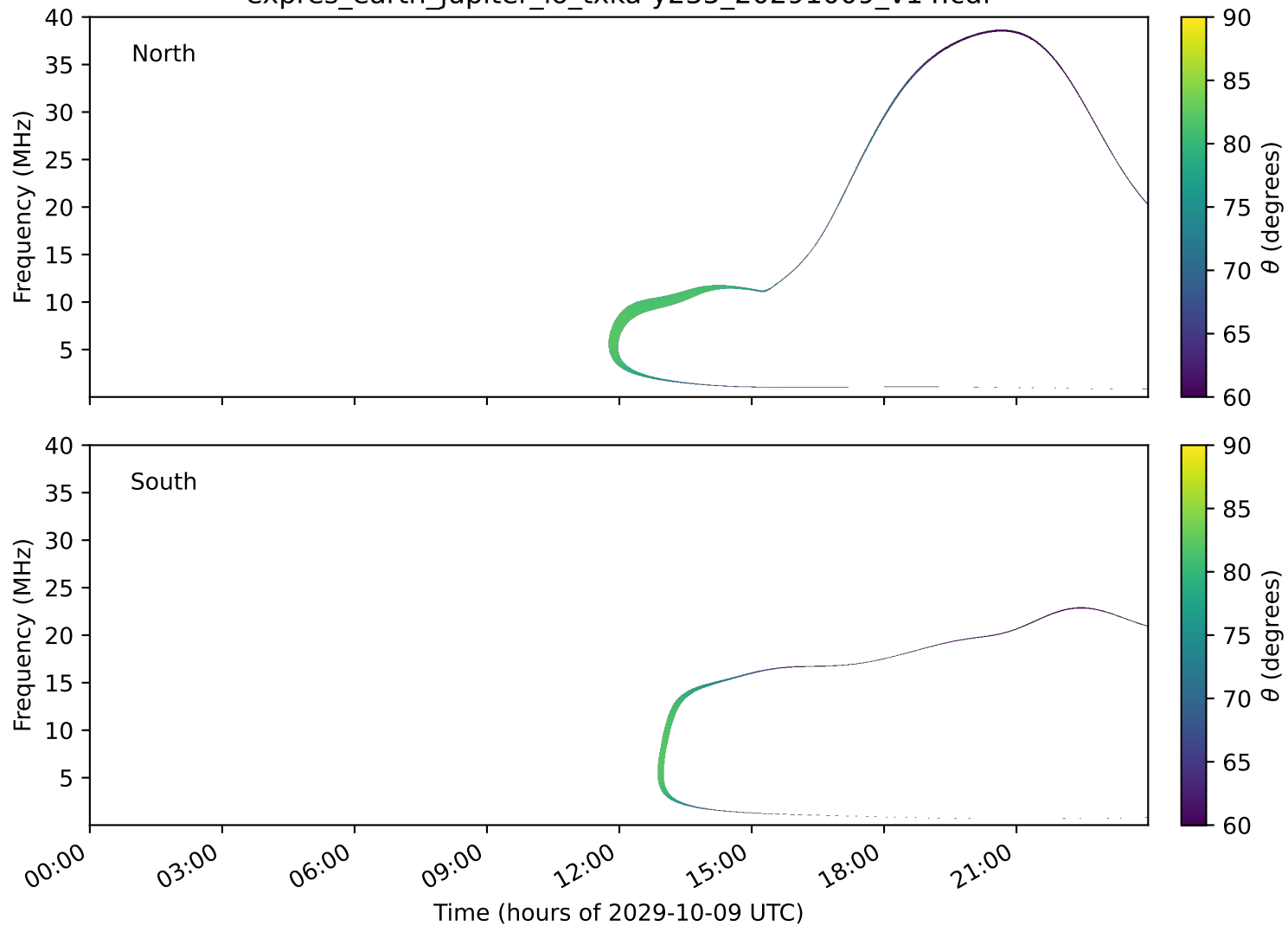
expres_earth_jupiter_io_txka-y235_20291009_v14.cdf
