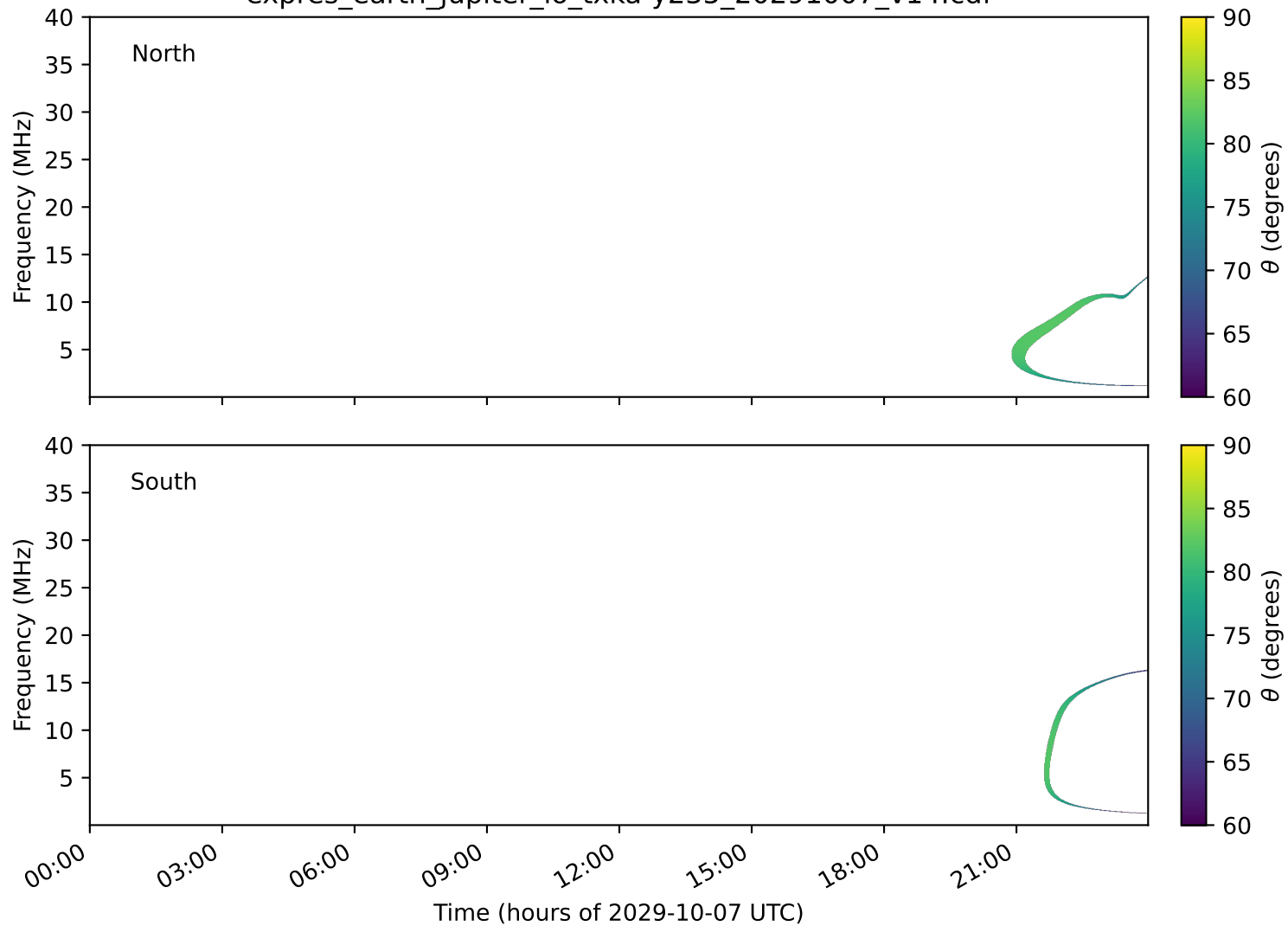
expres_earth_jupiter_io_txka-y235_20291007_v14.cdf
