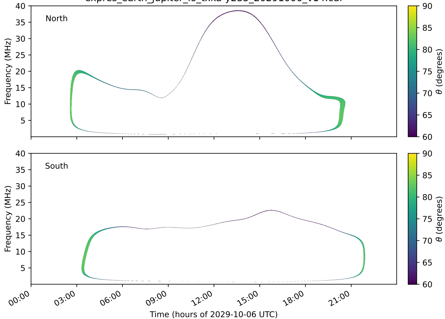
expres_earth_jupiter_io_txka-y235_20291006_v14.cdf
