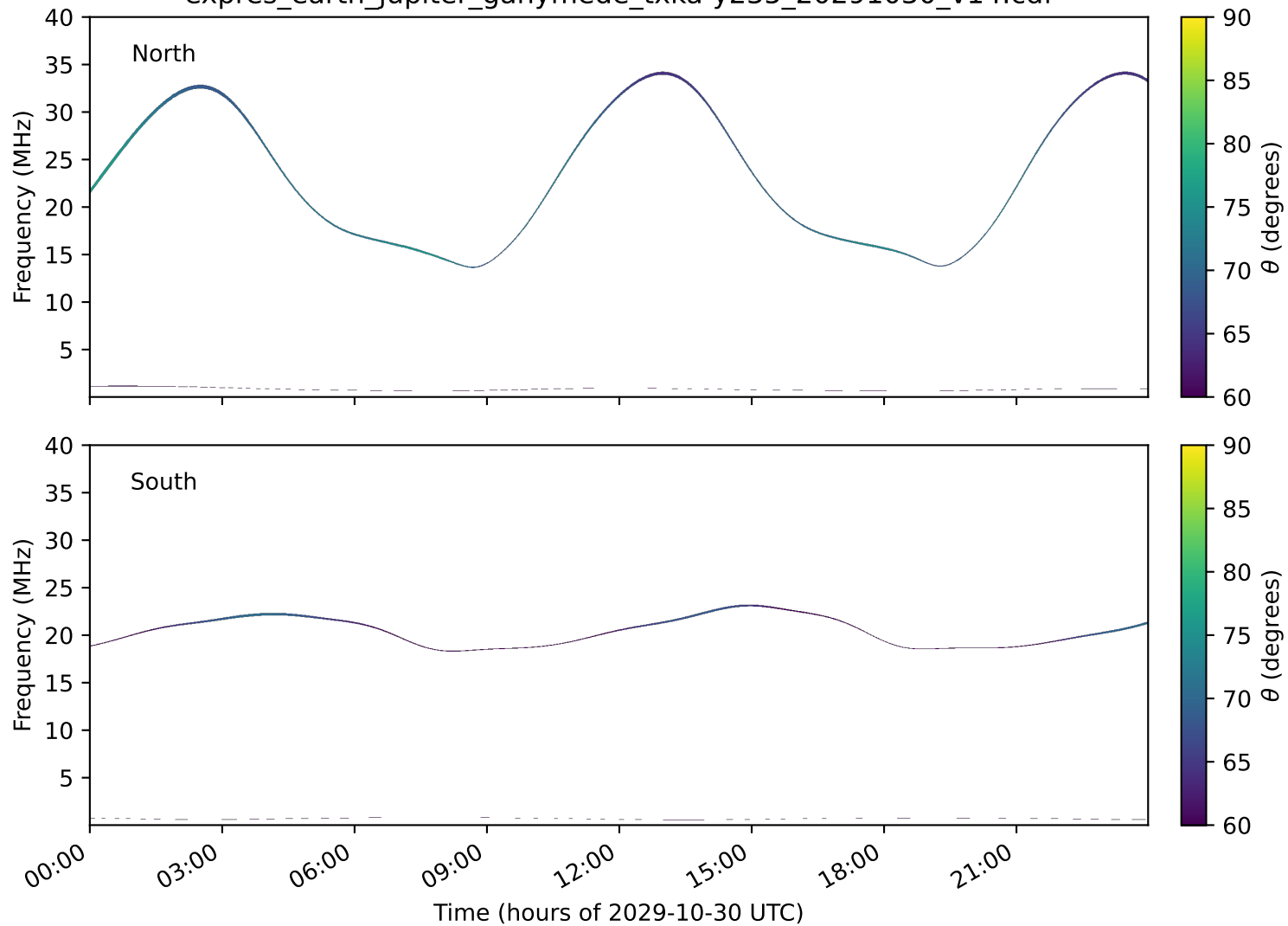
expres_earth_jupiter_ganymede_txka-y235_20291030_v14.cdf
