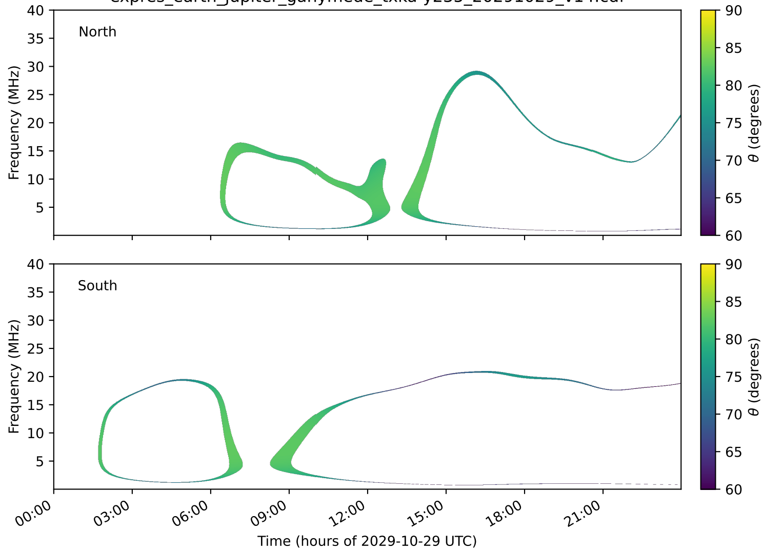
expres_earth_jupiter_ganymede_txka-y235_20291029_v14.cdf
