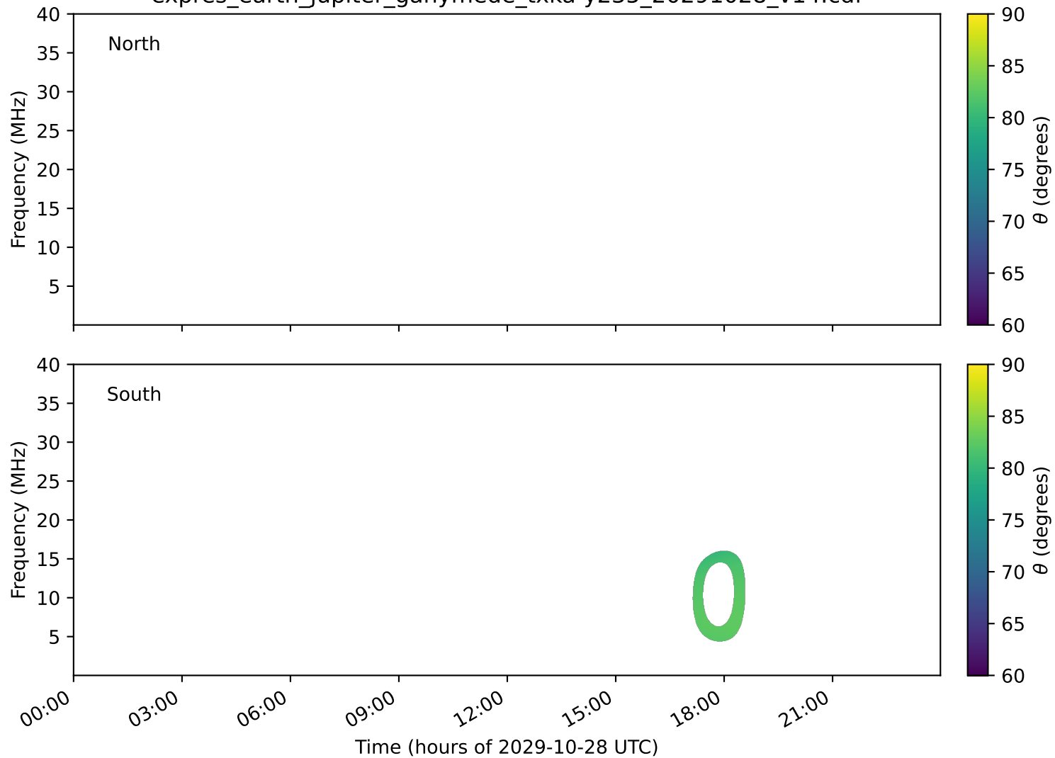
expres_earth_jupiter_ganymede_txka-y235_20291028_v14.cdf
