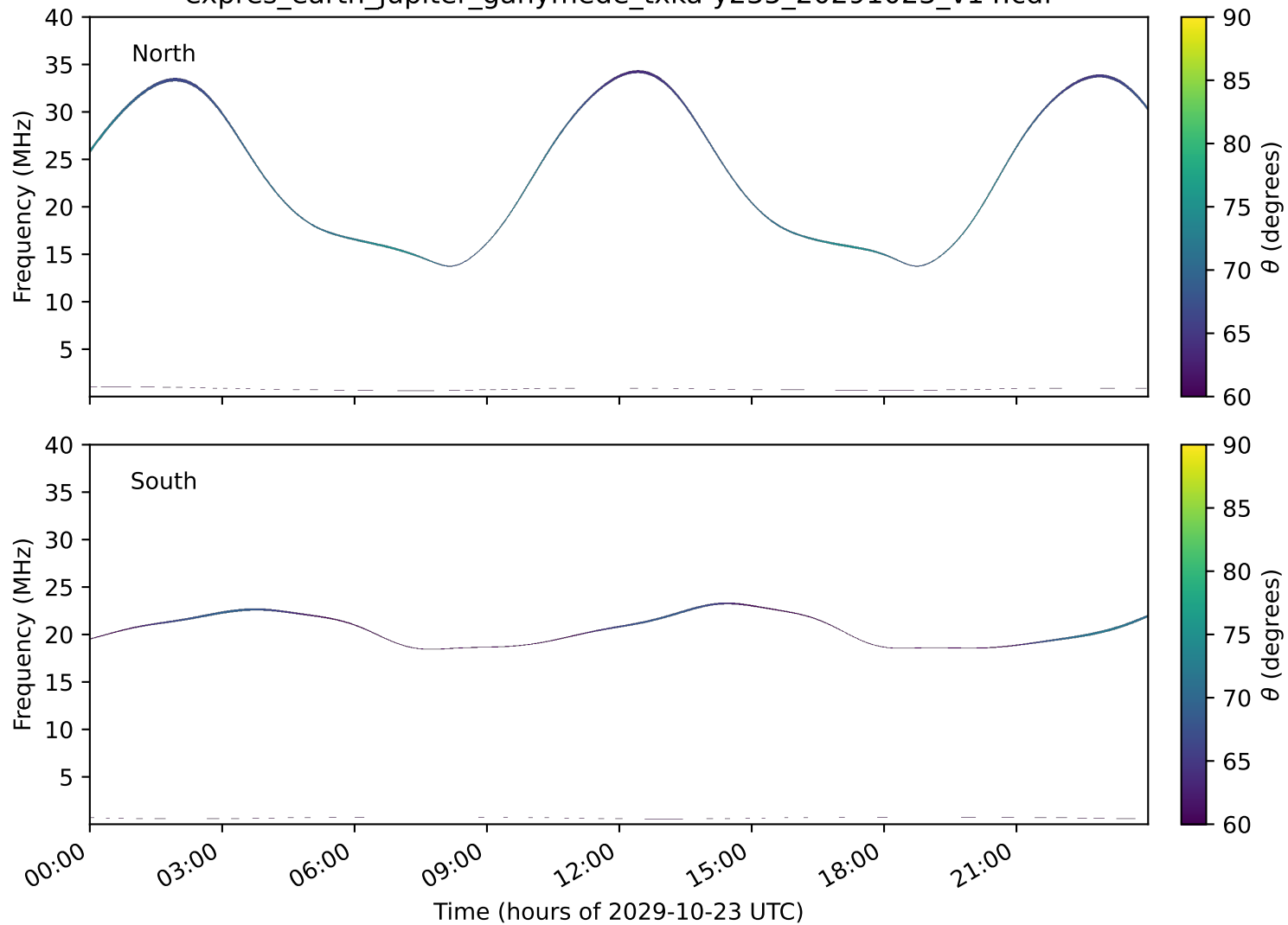
expres_earth_jupiter_ganymede_txka-y235_20291023_v14.cdf
