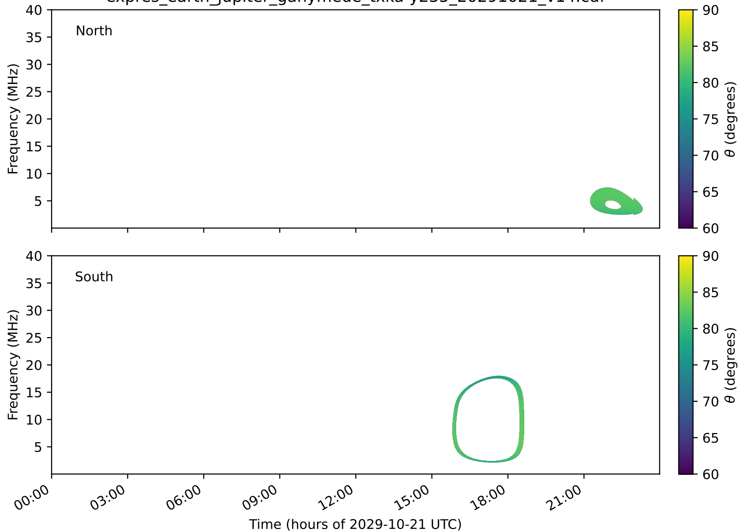
expres_earth_jupiter_ganymede_txka-y235_20291021_v14.cdf
