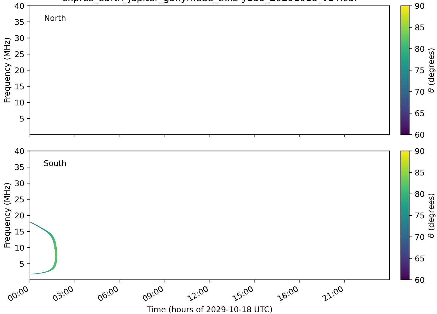
expres_earth_jupiter_ganymede_txka-y235_20291018_v14.cdf
